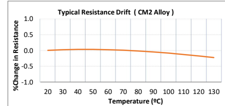
Resistance Change vs Temperature
