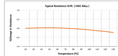
Resistance Change vs Temperature
