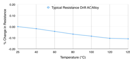
Resistance Change vs Temperature
