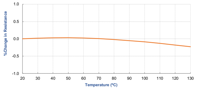
Typical Resistance Drift ( CM1 Alloy )
