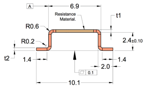
Mechanical Dimensions (mm)
