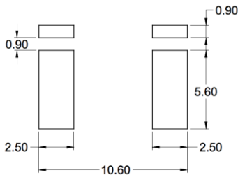
PCB Layout (Solder Pads) (mm)
