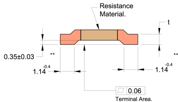
Mechanical Dimensions (mm)
