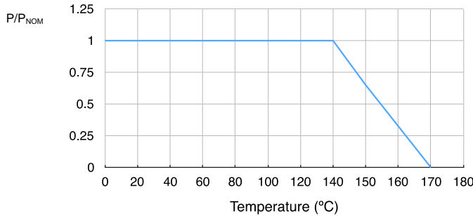
Power Derating Curve 4
