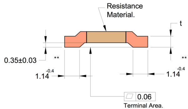
Mechanical Dimensions (mm)
