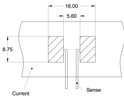
PCB Layout (Solder Pads) (mm)
